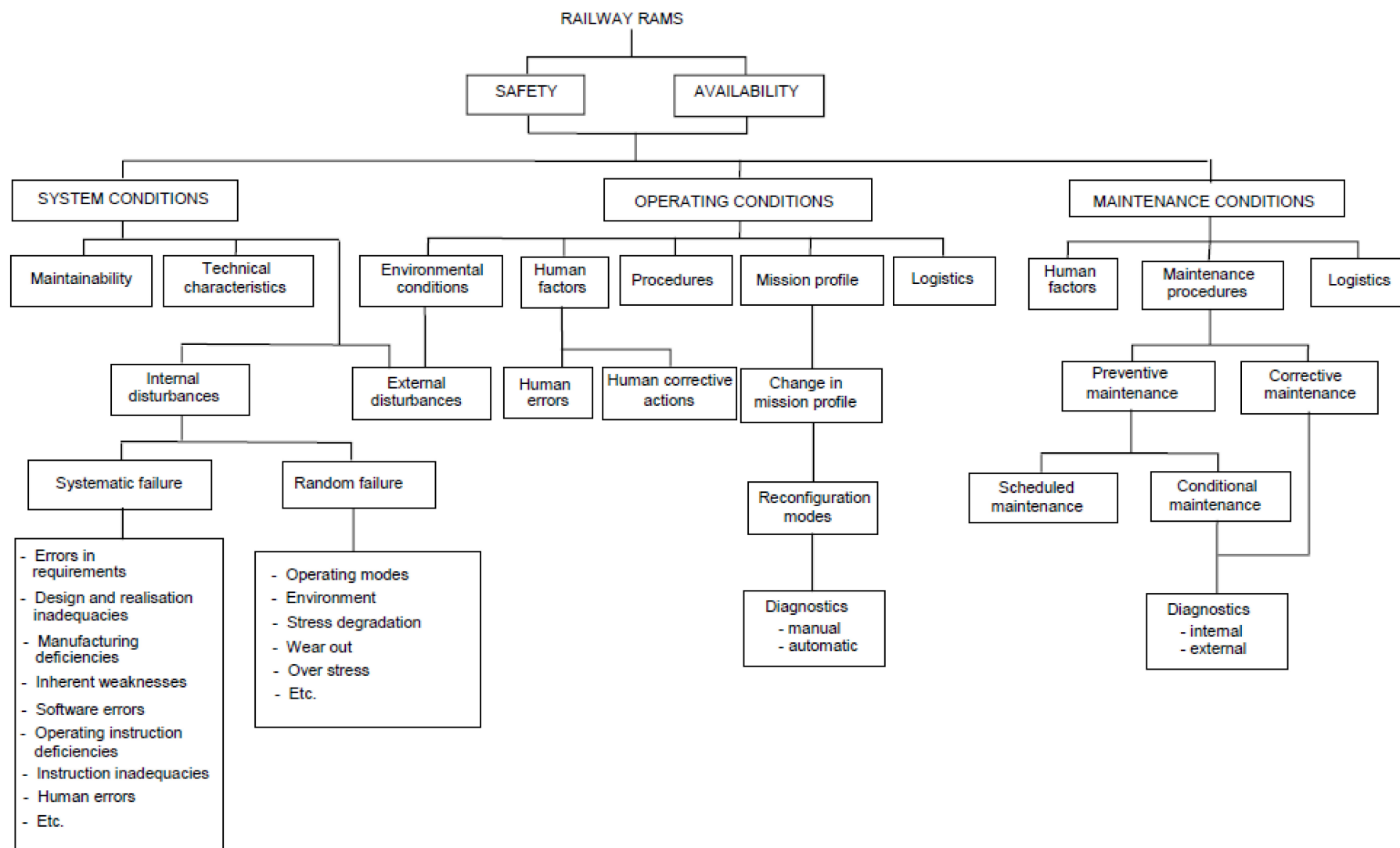
Figure 4 — Factors Influencing Railway RAMS
